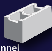
Hollow - three quarter 290x190x190mm Code 20-02
