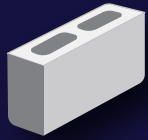
Hollow - Full Length 390x90x190mm Code 10-01
